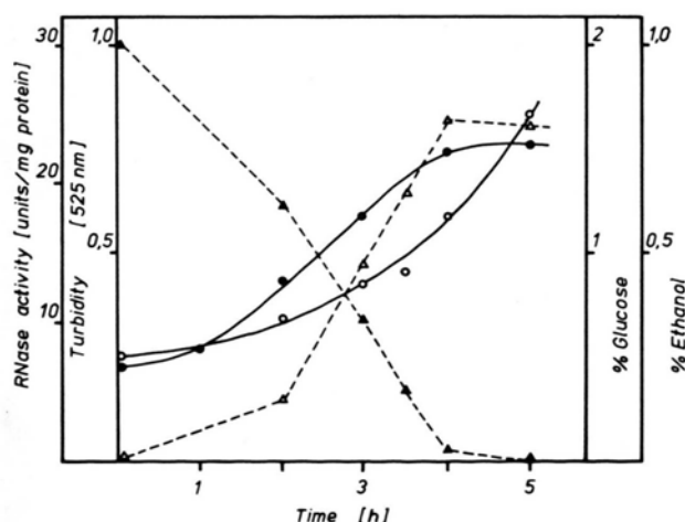
Fig. 2. Decrease of glucose concentration and increase of ethanol concentration and ribosomal ribonuclease activity during growth of yeast. ●—● turbidity (525 nm), ○—○ ribonuclease activity, ▲—▲ glucose concentration, △—△ ethanol concentration. (Medium: 0.5% pepton, 1% Difco yeast extract, 2% glucose.)
